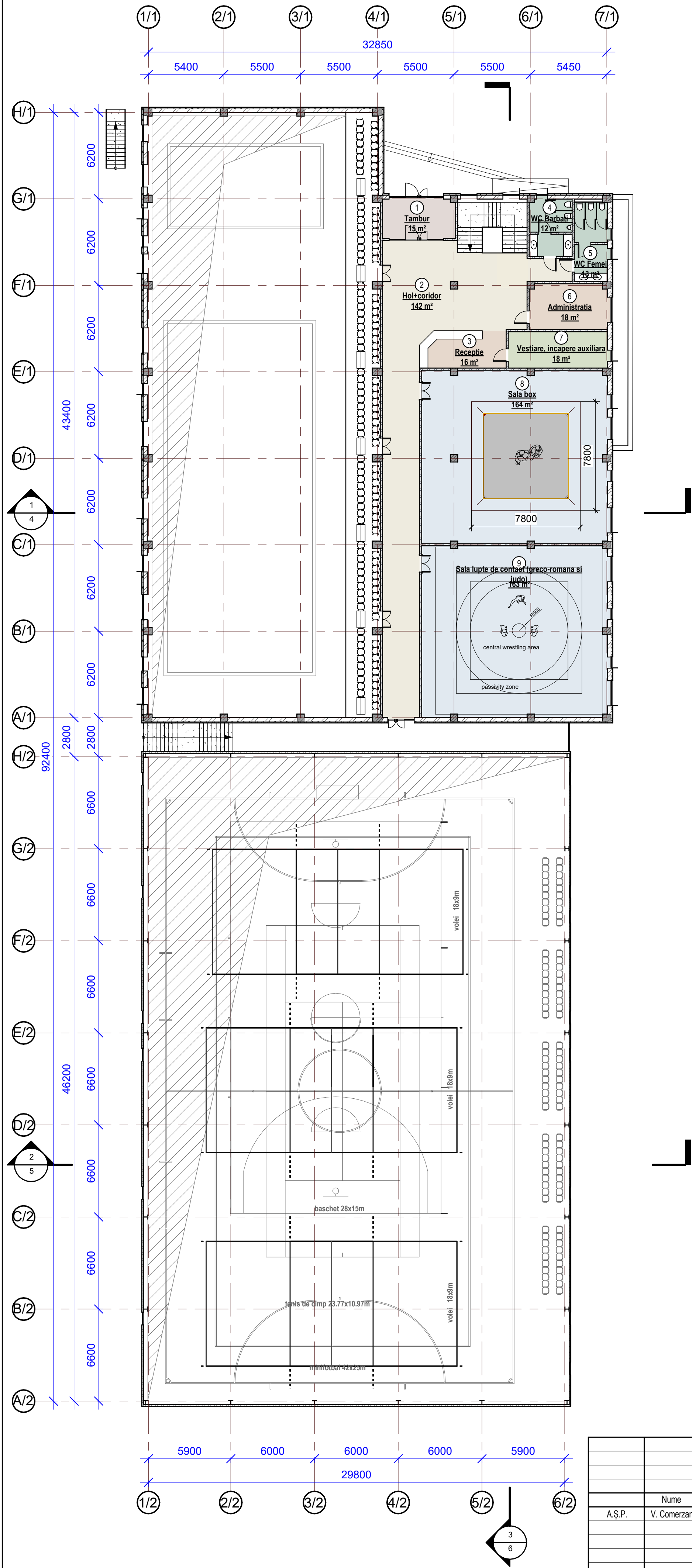
Plan parter (cota 0.000), sc. 1:200
